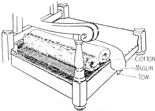
FIG. 478. WADDING.
